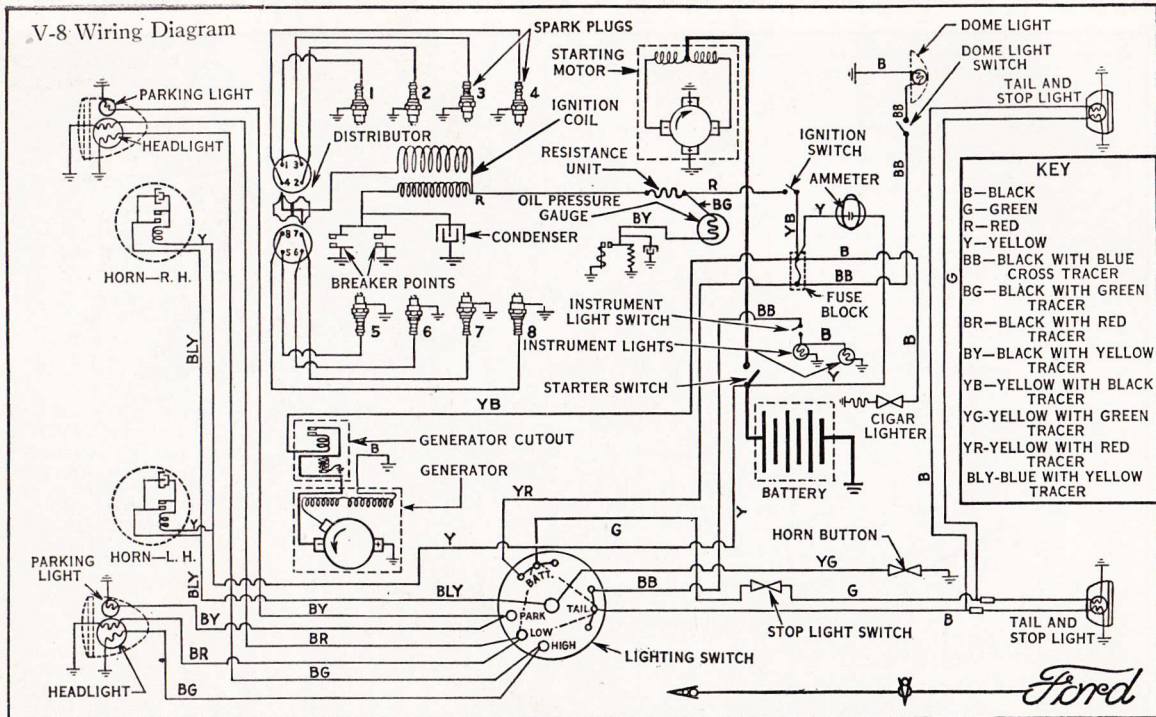
Fig. 84.—Technical Wiring Diagram of 1935 De Luxe Ford V8 Cars Showing All Circuits of Late Model Cars Excepting that of Electrical Fuel Tank Gauge. (See Fig. 110A Also)
